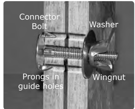
Connector Bolts
