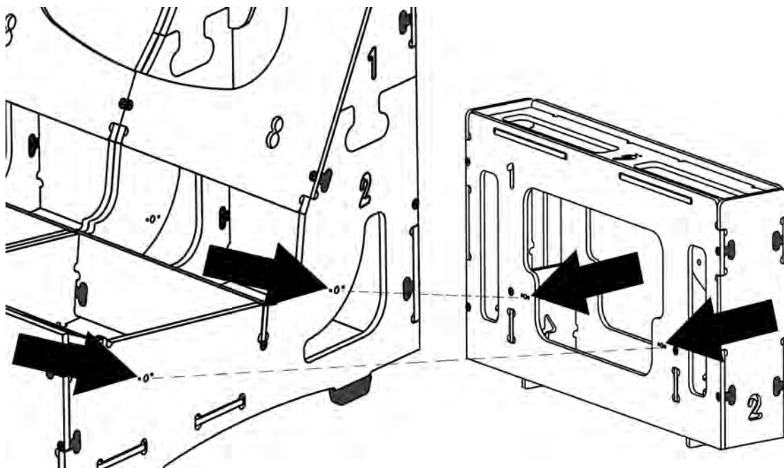
Connector Bolts
