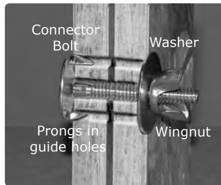
Connector Bolts
